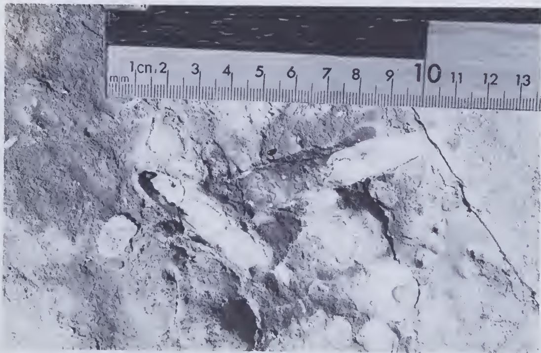
Fig. 4. Casts of belemnites, probably Dimitobelus sp. No internal structure is present in the casts; their composition appears to be identical to the phosphatic nodules lying adjacent to them.
